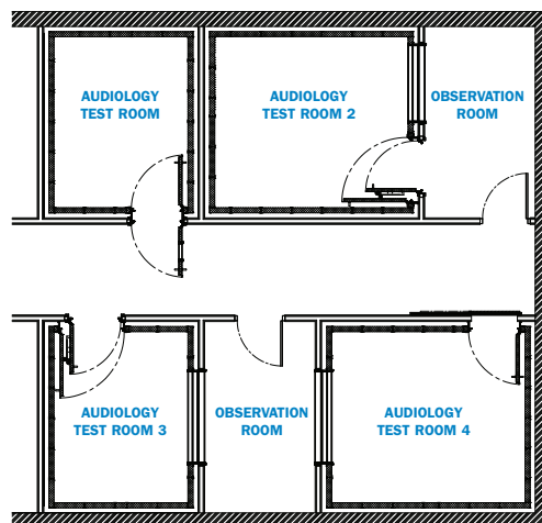
Typical layout of a 4-room turnkey audiometric suite
