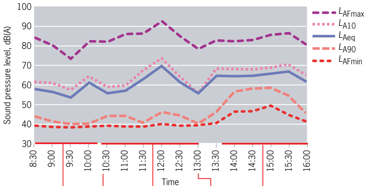
Figure 7.10.5: Learning base 1 – sound pressure levels in area A
