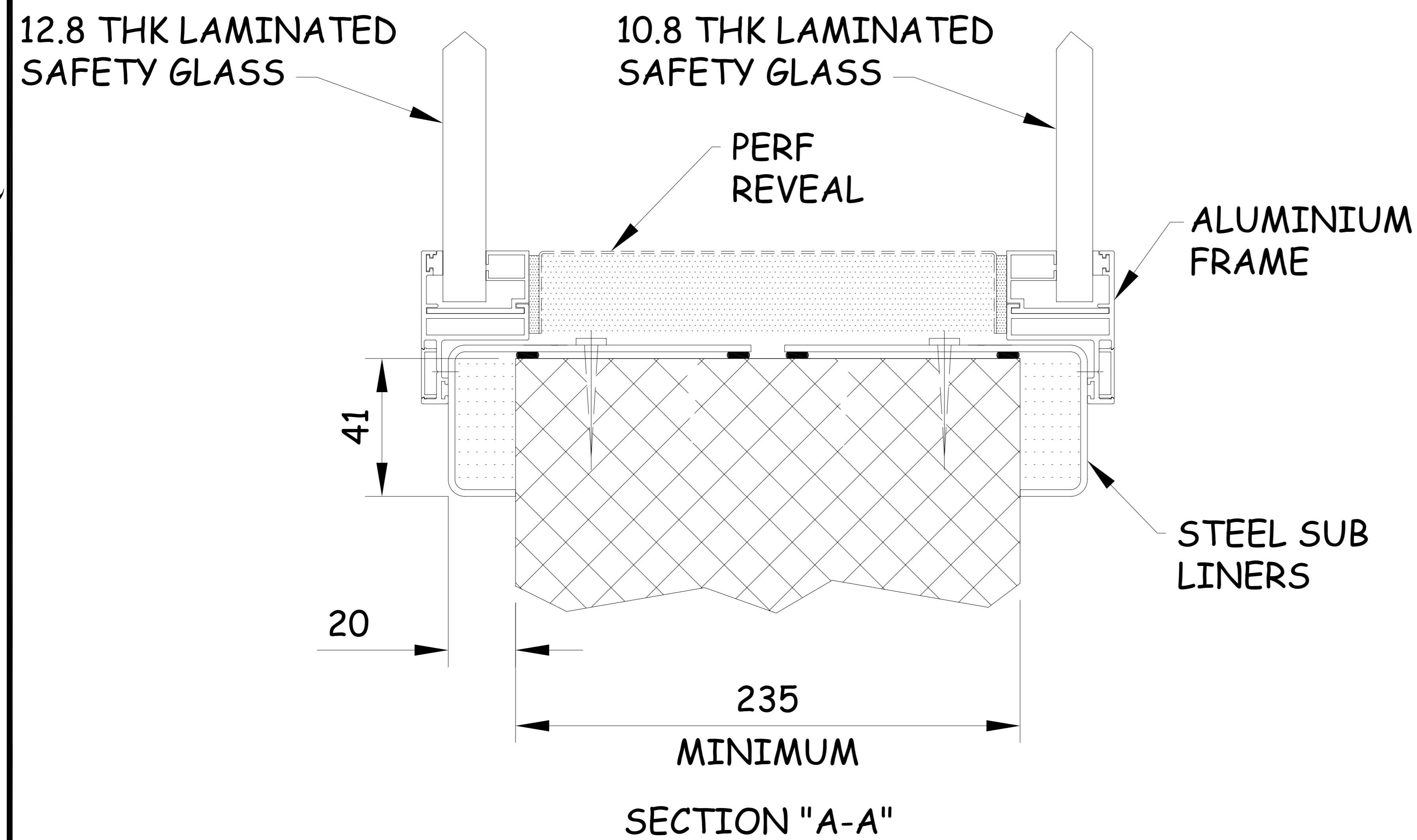
VERTICAL MULLION DETAIL
