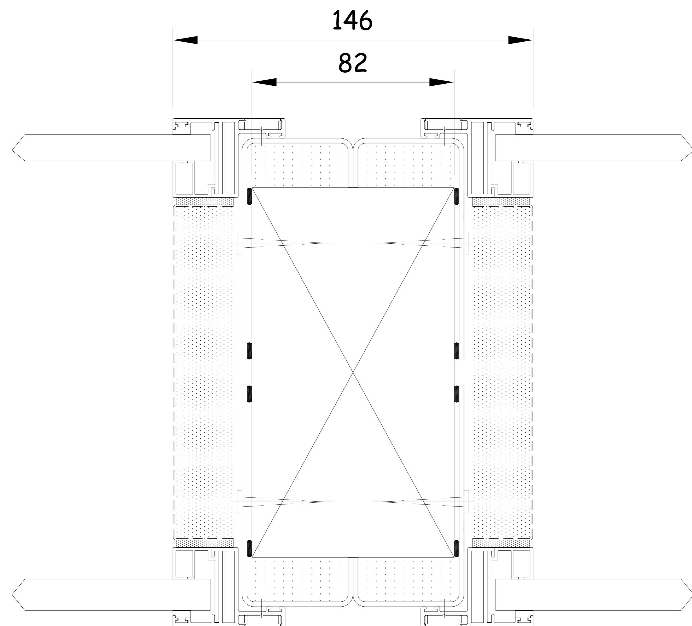
VERTICAL MULLION DETAIL
